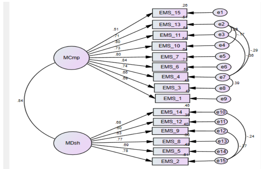
Figure 2: CFA Model of EMS Scale (N = 206)
